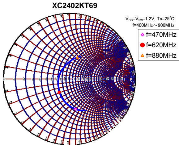
(28) Input Return Loss vs. Frequency (Smith Chart)
