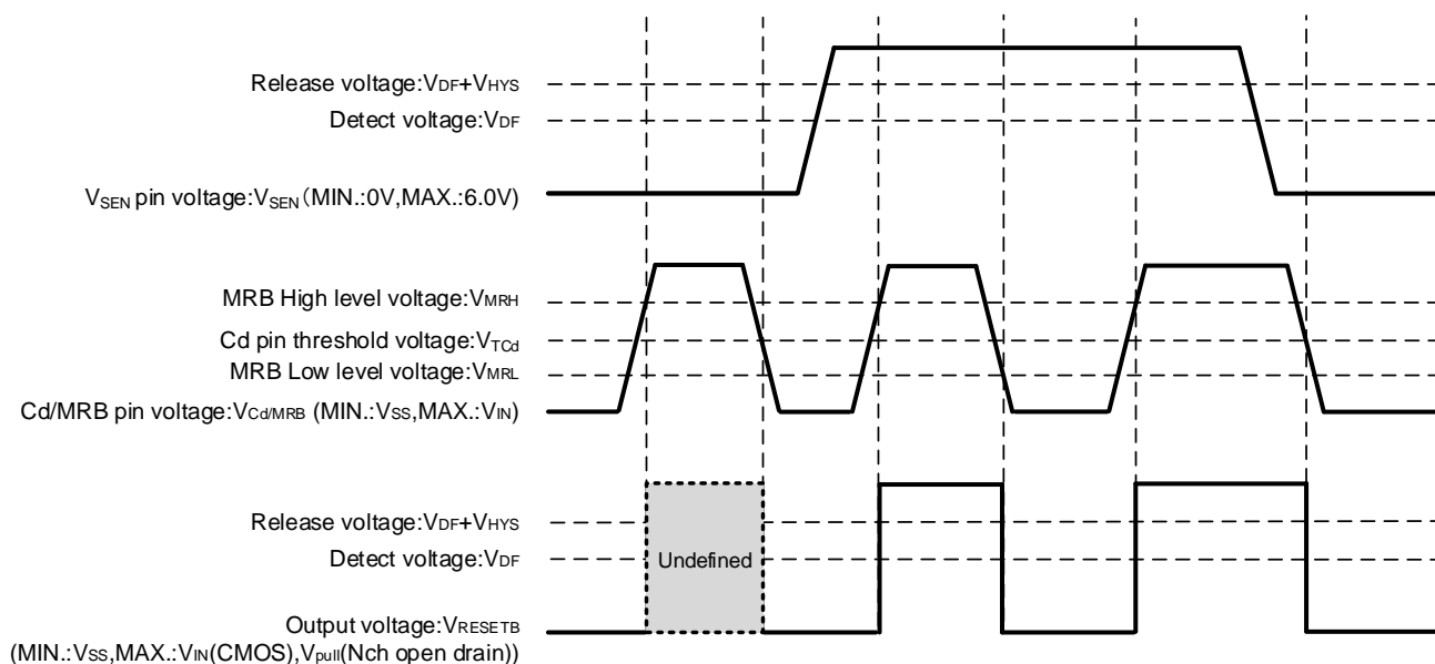
Fig. 4: Manual reset operation using the Cd/MRB pin ( V_{IN}=6.0V , Active Low)
